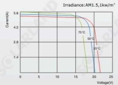
SLP085-12U I-V Curves
