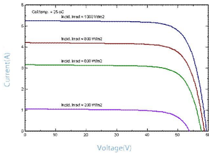
IV-CURVES of PV module SL230TU-48SP
