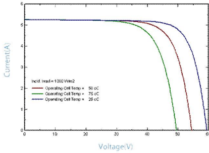
IV-CURVES of PV module SL225TU-48SP
