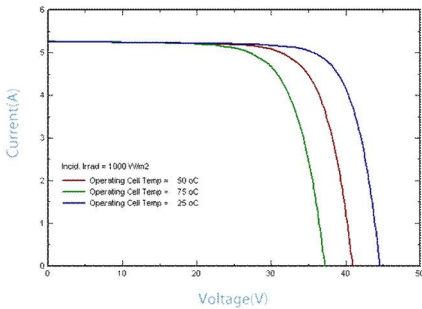
IV-CURVES of PV module SL165TU-36SP
