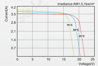
SLP055-12U I-V Curves
