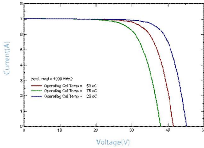
IV-CURVES of PV module SL250TU-36CM
