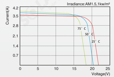
SLP050-12U I-V Curves
