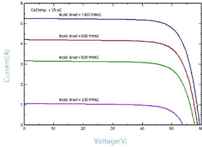
IV-CURVES of PV module SL250TU-48SP
