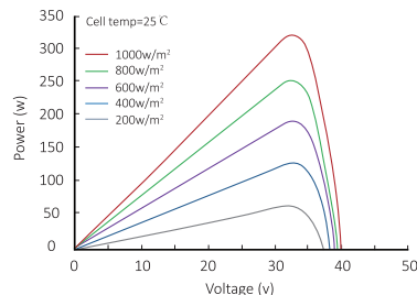
Power-Voltage Curve (LR6-60HPH-320M)
