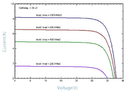
IV-CURVES of PV module SL205TU-27P
