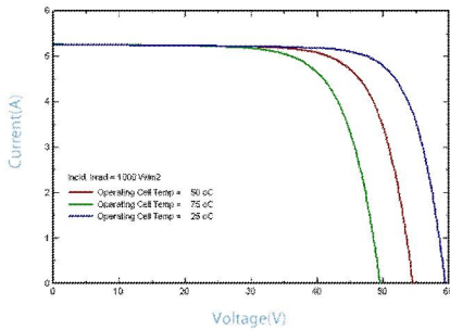
IV-CURVES of PV module SL240TU-48SP
