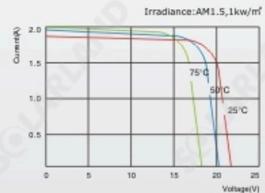
SLP030-12 I-V Curves
