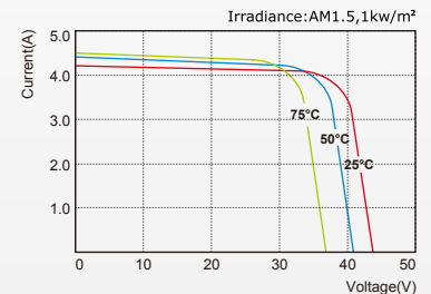
SLP140-24 I-V Curves
